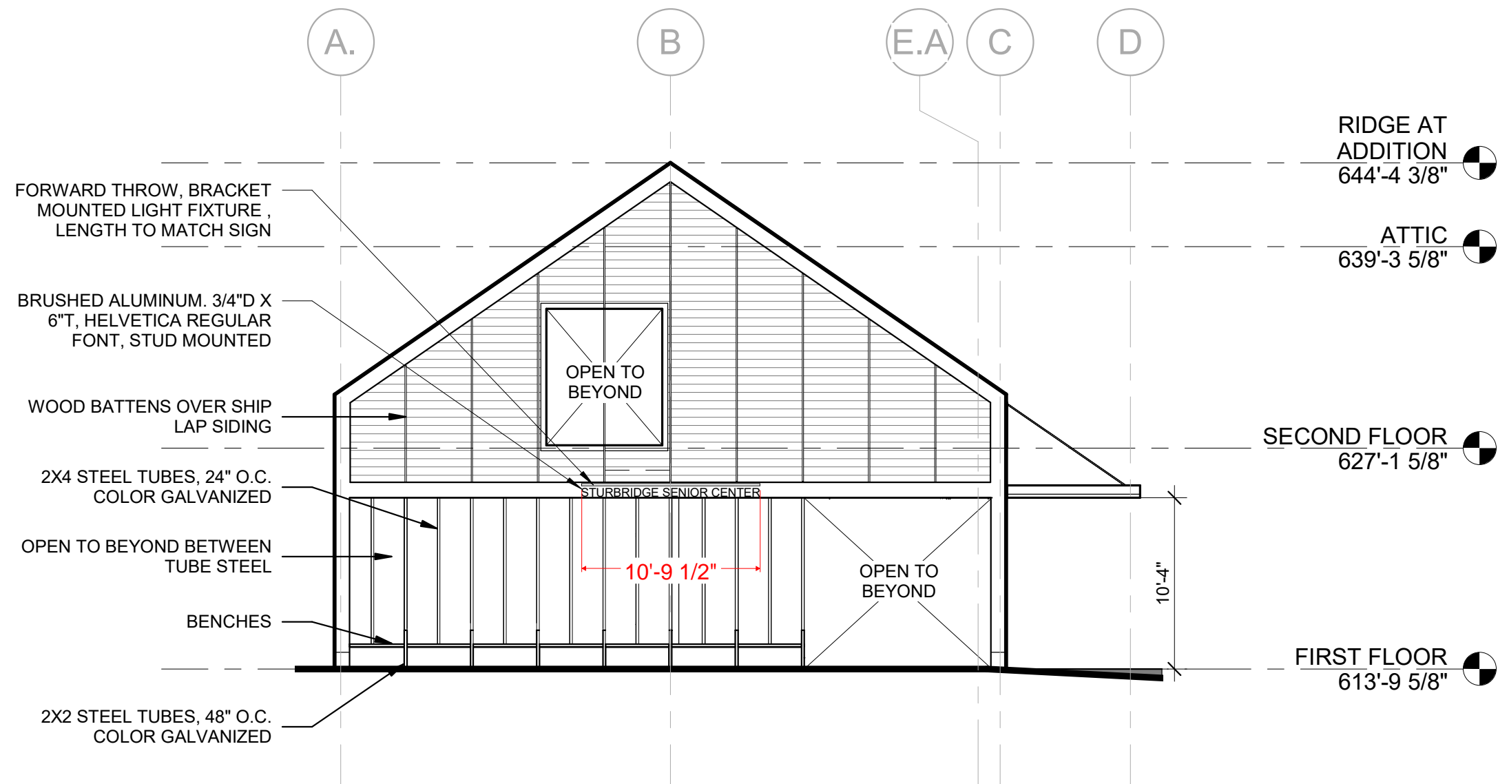
1 WEST ELEVATION - PORTE COCHERE 1/8" = 1'-0"
