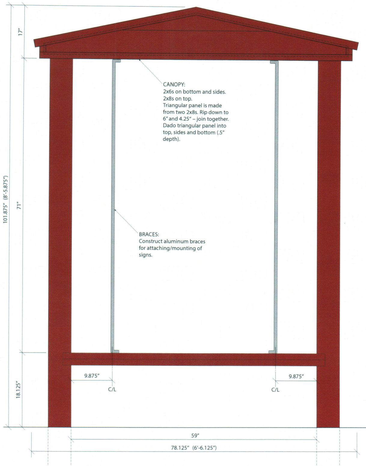
- ELEVATION, SIGN FRAMING -
