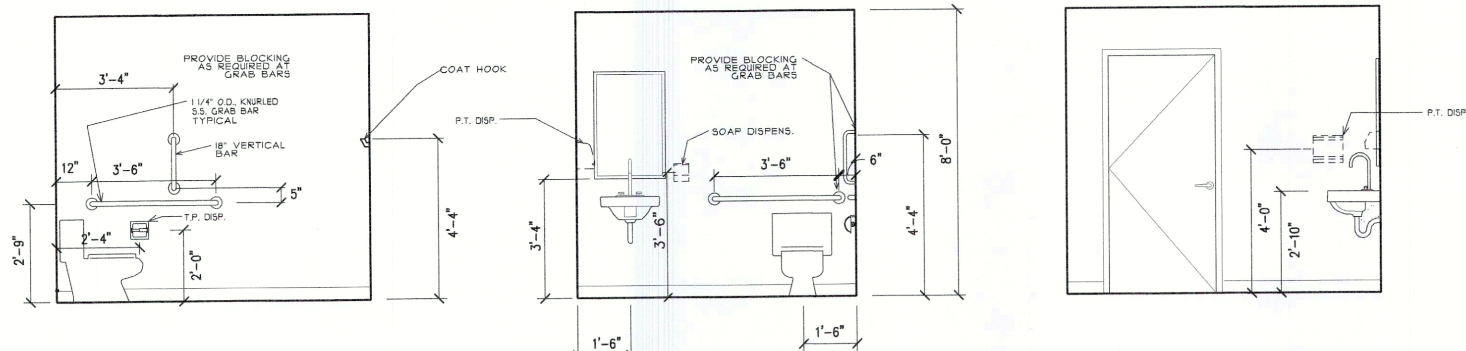
REST ROOM ROOM ELEVATIONS SCALE: 3/8"=1'-0"
