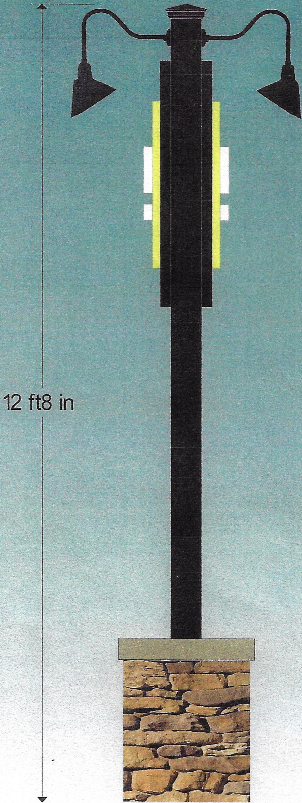
Side View
