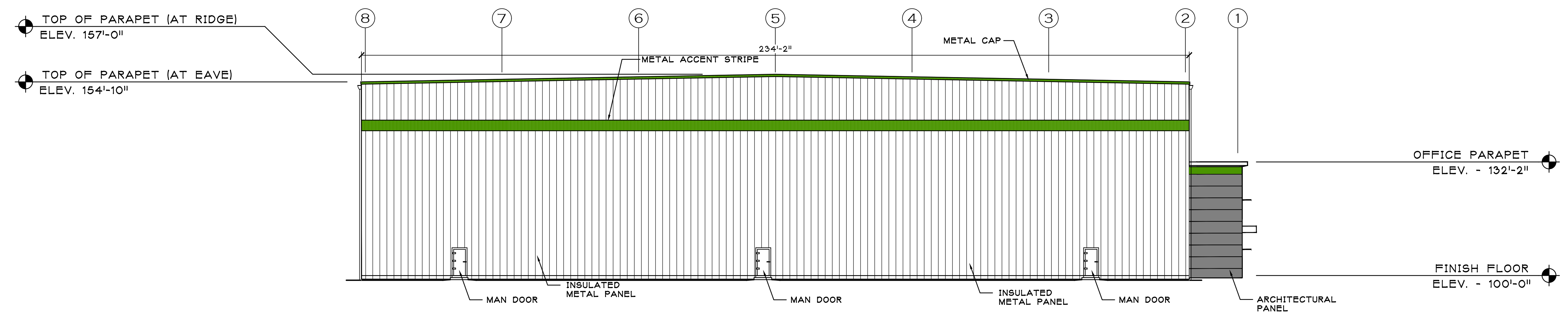
3 NORTH BUILDING ELEVATION SCALE: 1/16" = 1'-0" AT WAREHOUSE
