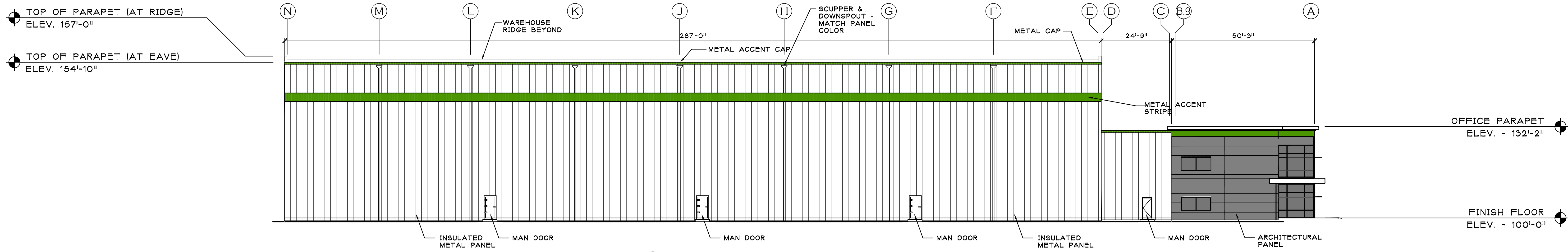
2 WEST BUILDING ELEVATION SCALE: 1/16" = 1'-0" AT WAREHOUSE, DOCK AND OFFICE
