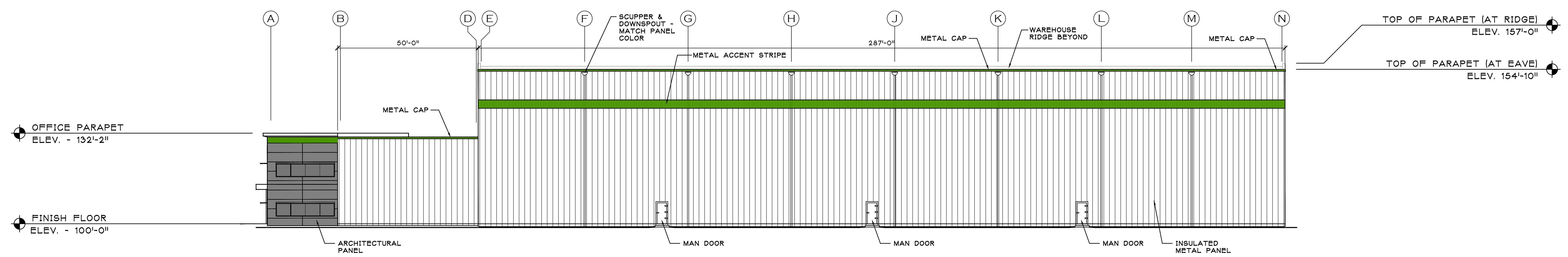
4 EAST BUILDING ELEVATION SCALE: 1/16" = 1'-0" AT WAREHOUSE & DOCK
