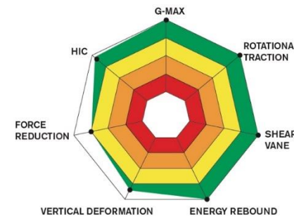
Legion 2.0 with Sand/Rubber
